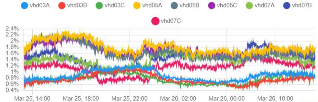
Voltage Harmonics (3, 5, 7)
