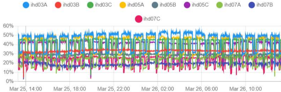
Current Harmonics (3, 5, 7)
