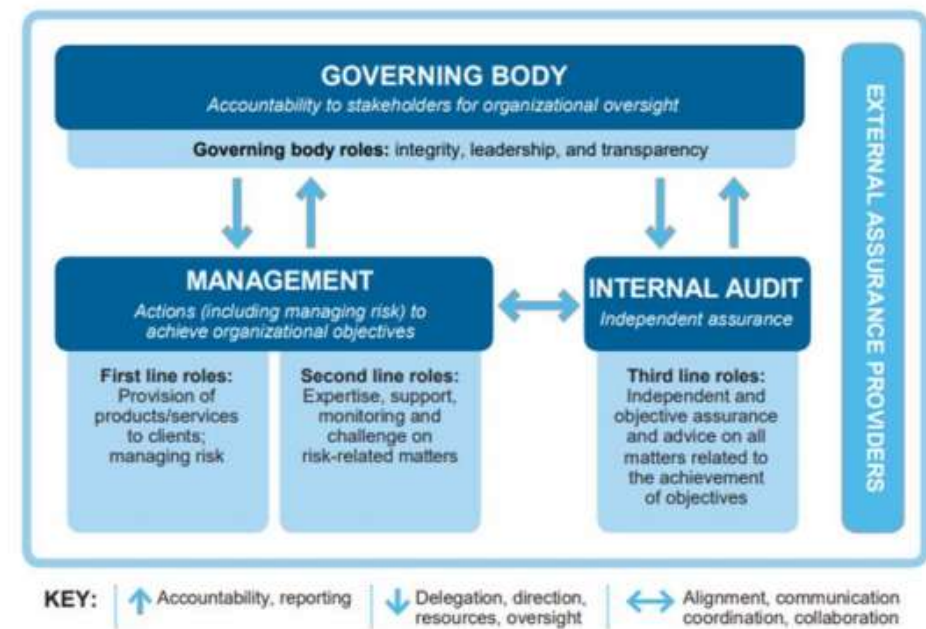
Fig 2: The new Three Lines Model
